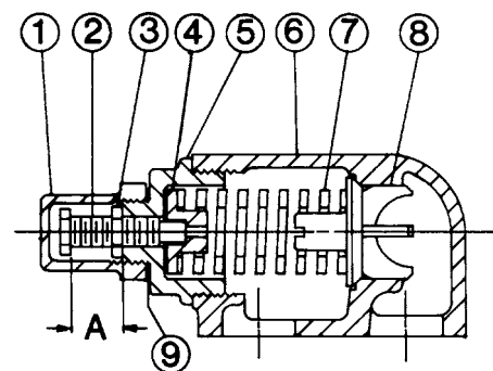
FIGURE 8 CLAPET - TAILLE G
